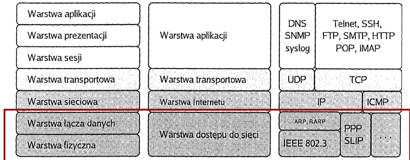
Model ISO/OSI
