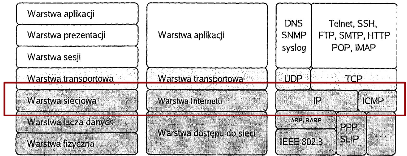
Model ISO/OSI
