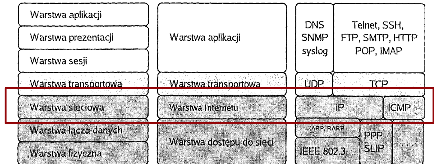
Model ISO/OSI
