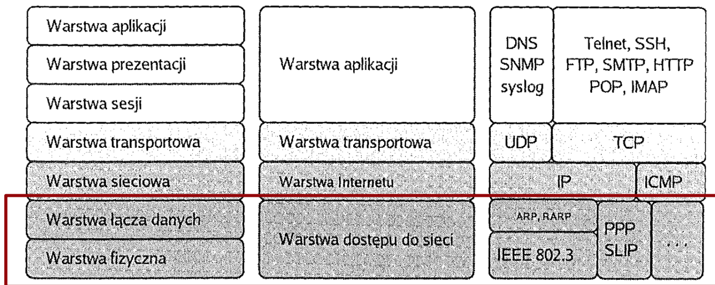
Model ISO/OSI
