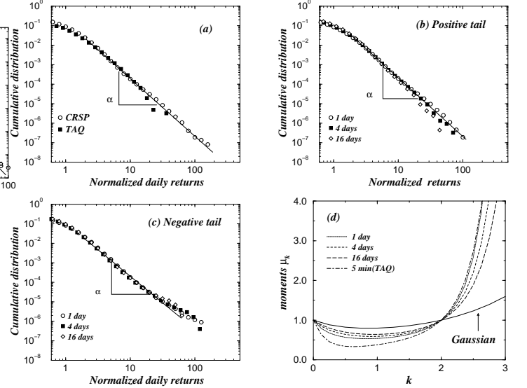
FIG. 8. (a) Cumulative distribution of normalized daily returns computed from the CRSP database contrasted with the same distribution from the TAQ database, normalized by the average volatility. Regression fits yield estimates \alpha = 2.96 \pm 0.09 (positive tail), and \alpha = 2.70 \pm 0.10 (negative tail) for the CRSP data, and \alpha = 3.27 \pm 0.19 (positive tail) and \alpha = 2.98 \pm 0.21 (negative tail) for the TAQ data. The regression fits were performed for the region 2 \leq g \leq 80 . (b) Positive and (c) negative tails of the cumulative distribution of normalized returns for \Delta t = 1, 4 and 16 days. Estimates of the exponents are listed in Table I. (d) The fractional moments \mu_k \equiv \langle |g|^k \rangle for the normalized returns for the same time scales. The thick full line shows the Gaussian moments.
