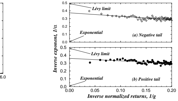
FIG. 3. The inverse local slope of P(g) , \zeta^{-1}(g) \equiv -(d \log P(g)/d \log g) as a function of the inverse normalized returns 1/g for (a) the negative tail and (b) the positive tail [16,27]. Each data point shown is an average over 1000 events and the lines are linear regression fits to the data. The linear regression fit over the range 0 \leq g \leq 0.2 yields the values of the inverse asymptotic slopes, 1/\alpha ; we find, \alpha = 2.84 \pm 0.12 for the positive and \alpha = 2.73 \pm 0.13 for the negative tail. Note that the average over all events used would be identical to the estimator for the asymptotic slope proposed by Hill [27].
