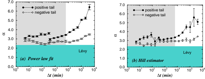
FIG. 10. The values of the exponent \alpha characterizing the asymptotic power-law behavior of the distribution of returns as a function of the time scale \Delta t obtained using (a) a power-law fit, and (b) the Hill estimator. The values of \alpha for \Delta t < 1 day are calculated from the TAQ database while for \Delta t \geq 1 day they are calculated from the CRSP database. The unshaded region, corresponding to time scales larger than (\Delta t)_\times \approx 16 days (6240 min), indicates the range of time scales where we find results consistent with slow convergence to Gaussian behavior.
