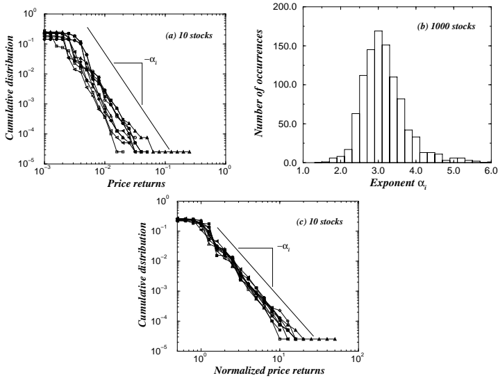
FIG. 1. (a) Cumulative distributions P(g > x) for the positive tails of 10 randomly-selected companies. Note that they are all consistent with a power-law asymptotic behavior. (b) The histogram of the power-law exponents obtained by power-law regression fits to the individual cumulative distribution functions, where the fit is for all x larger than 2 standard deviations. Note that this histogram is not normalized—the y-axis indicates the number of occurrences of the exponent. (c) Cumulative distributions of the 10 randomly chosen companies in (a) scaled by the standard deviation calculated from the entire 2-year period.
