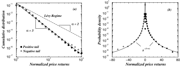
FIG. 2. (a) Cumulative distributions of the positive and negative tails of the normalized returns of the 1000 largest companies in the TAQ database for the 2-year period 1994–1995. The solid line is a power-law regression fit in the region 2 \leq x \leq 80 . (b) Probability density function of the normalized returns. The values in the center of the distribution arise from the discreteness in stock prices, which are set in units of fractions of USD, usually 1/8 , 1/16 , or 1/32 . The solid curve is a power-law fit in the region 2 \leq x \leq 80 . We find \alpha = 3.10 \pm 0.03 for the positive tail and \alpha = 2.84 \pm 0.12 for the negative tail.
