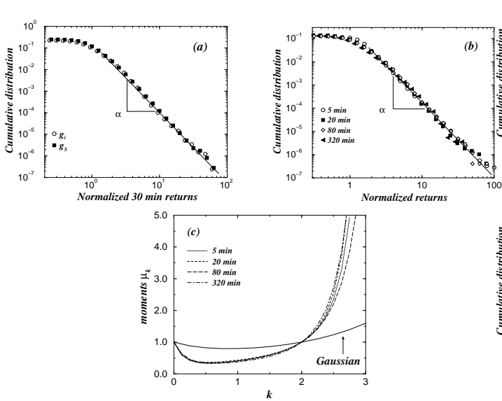
FIG. 6. (a) Cumulative distribution of normalized returns for \Delta t = 30 min. The filled squares show the distribution for returns normalized by the time-averaged volatility for each company, as defined in Eq. (5). The circles show the distribution for returns normalized by the average volatility for each size bin, Eq. (10), showing the consistency of these two methods. (b) The distribution of returns for different time scales \Delta t \leq 1 day. The exponents from the power-law regression fits are summarized in Table I. (c) Fractional moments from 0 \leq k < 3 for the normalized returns for the same scales as in (b). Note that the moments are not converging to Gaussian behavior, for example, at large k the moments for \Delta t = 80 min is to the right of \Delta t = 320 min. The thick full line shows the Gaussian moments.
