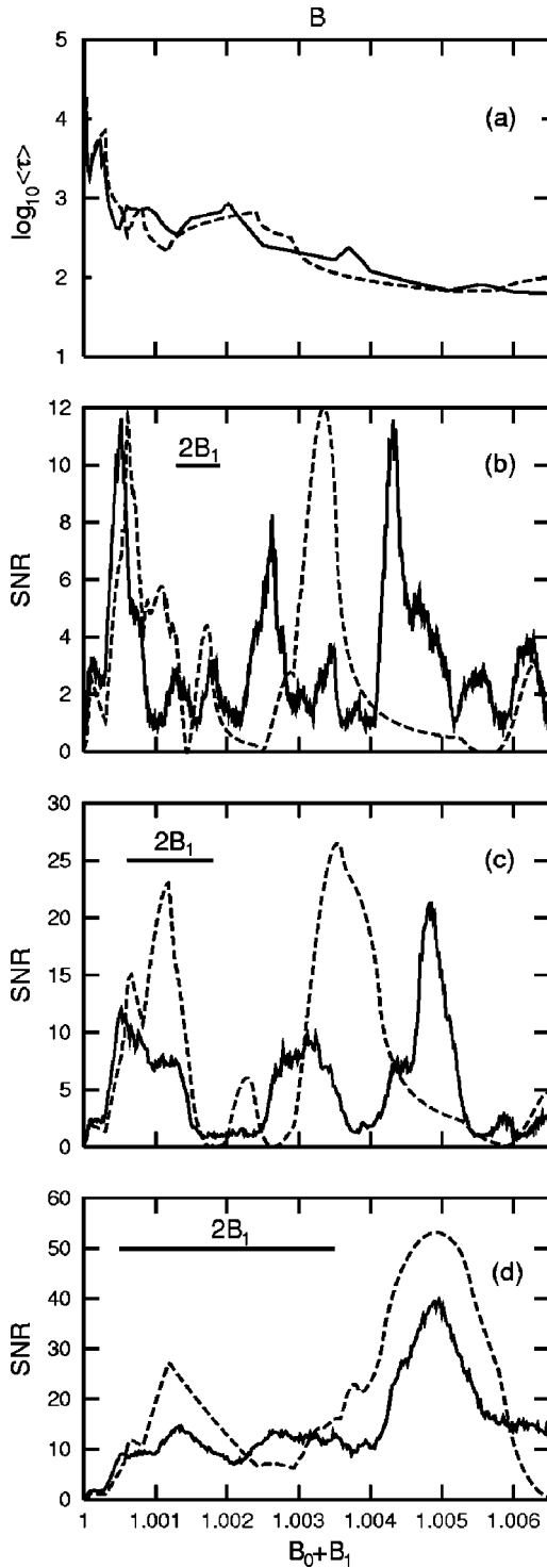
FIG. 7. (a) The mean time between jumps between symmetric parts of the attractor \langle \tau \rangle vs B for the spin map (6) with parameters as in Fig. 1. Numerical results are shown with solid line and theoretical results obtained from the theory of Sec. IV B with \alpha = 0.0108 , \gamma = 0.294 , \beta = 0.125 , b_E = 1.46793 , a/b = 1.667 , \zeta = 3.33 , and K = L = 10 —with dashed line. (b)–(d) The SNR vs B_0 + B_1 for the signal y_n from the spin map (6) with parameters as in Fig. 1 and T_0 = 1024 : (b) B_1 = 3 \times 10^{-4} , (c) B_1 = 6 \times 10^{-4} , (d) B_1 = 1.5 \times 10^{-3} . The solid lines show numerical results. The dashed lines show theoretical results evaluated from Eq. (9) with the parameters of the theory of Sec. IV B as in (a).
