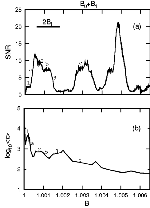
FIG. 3. (a) The SNR vs B_0 + B_1 for the signal y_n from the spin map (6) with parameters as in Fig. 1 and B_1 = 6 \times 10^{-4} , T_0 = 1024 . (b) The mean time between jumps between symmetric parts of the attractor \langle \tau \rangle vs B for the spin map (6) with parameters as in Fig. 1; anomalous oscillations can be seen. The labeled segments in (a) and (b) correspond to each other according to the heuristic rules discussed in Appendix A [segment 2 in (b) is a composite segment consisting of a rising and flat part].
