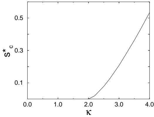
Fig. 4. Critical external support s_c^* (Eq. (27)) as a function of \kappa .
