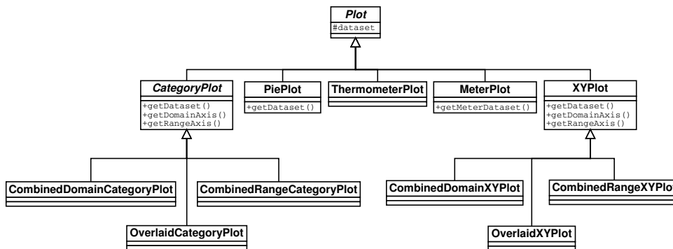
Figure 29.6: Plot classes
