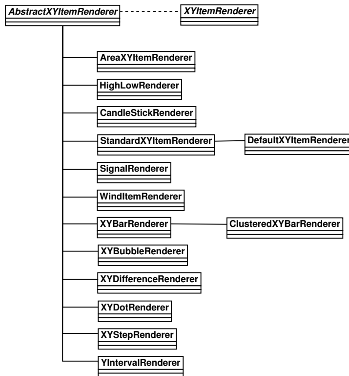
Figure 30.17: Renderer hierarchy
