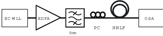
Figure 1: Experimental setup (abbreviations are defined in the text).
