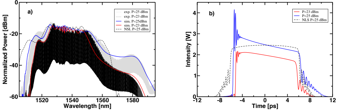
Figure 2: Spectra a) and pulse shapes b) for injected pulses with \text{sech}^2 forms with widths \tau_0 = 1.8\text{ps} and average powers P_{IN} of 23.0\text{dBm} and 25\text{dBm} after the HNLF at \lambda_p = 1535\text{nm} with dispersion coefficients \beta_2 = 0.53\text{ps}^2/\text{km} and \beta_3 = 0.03\text{ps}^3/\text{km} . The dashed black lines represent the simulation for the NLSE without TOD.
