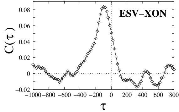
FIG. 2: Example for the measured shifted-time correlation function. The two companies are: Ensco International (ESV) and Exxon Corp. (XON). The maximum correlation value is at -100 sec, which means that the return time series of ESV has to be shifted back in order to get the maximal correlation i.e. the price changes happen later in time, in other words ESV is pulled by XON.
